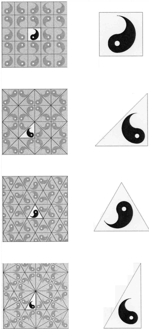
Chart 1. The four classic polygonal kaleidoscopes (infinite reflection).
